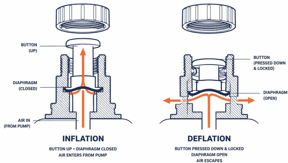
Fig. 3a · Push/push valve — inflation (button up, diaphragm closed) vs deflation (button locked down, diaphragm open).
