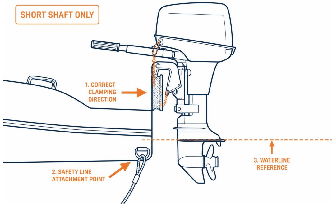
Fig. 5 · Outboard mounting — short shaft only, clamps even, safety line to transom D-ring.
