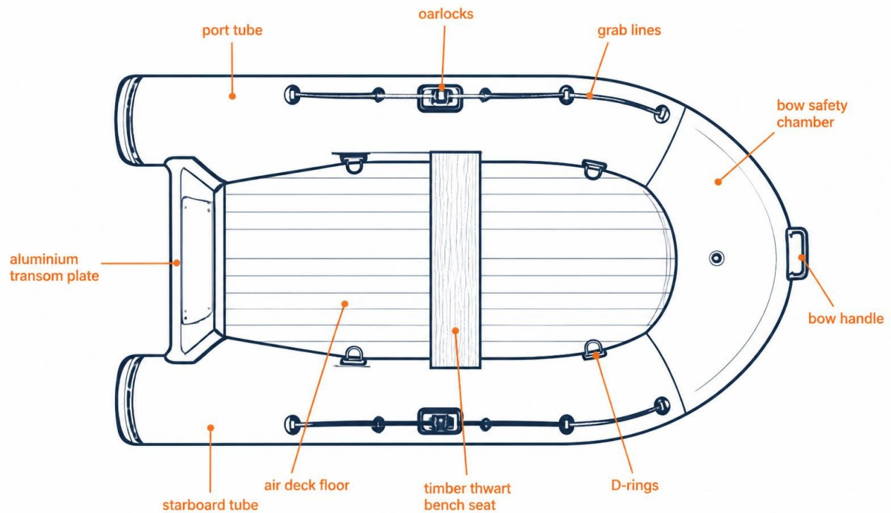
Fig. 1 · Swift Tender — parts and fittings (top view).
