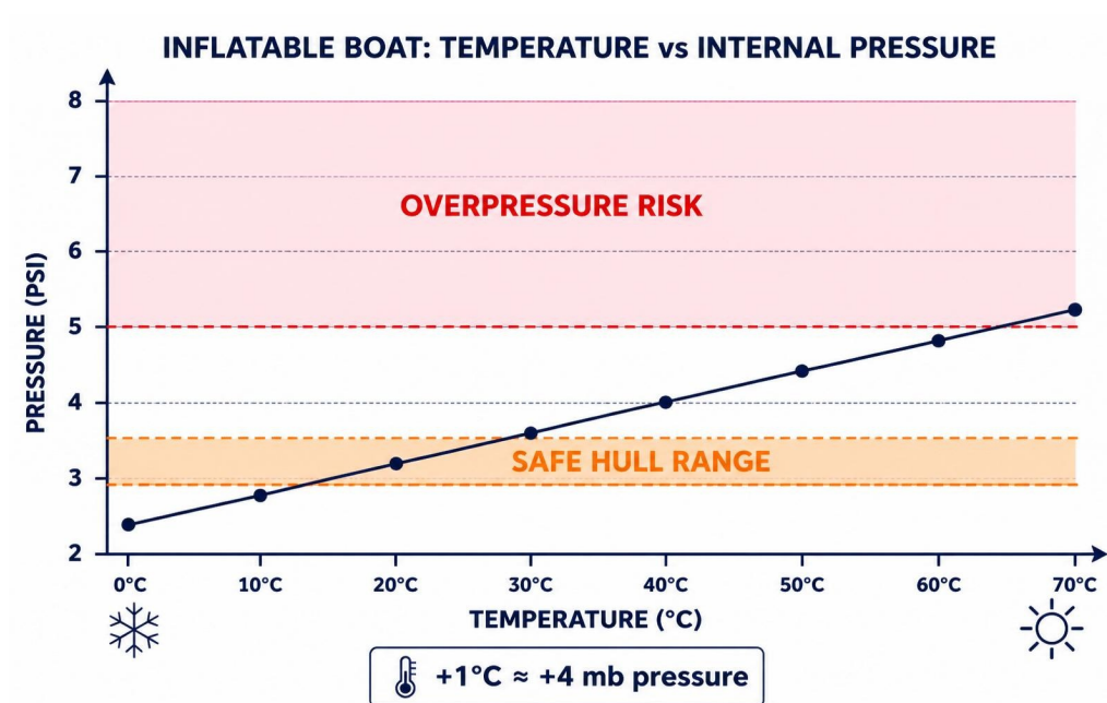
Fig. 4 · Temperature vs. internal pressure — check the gauge every launch.
