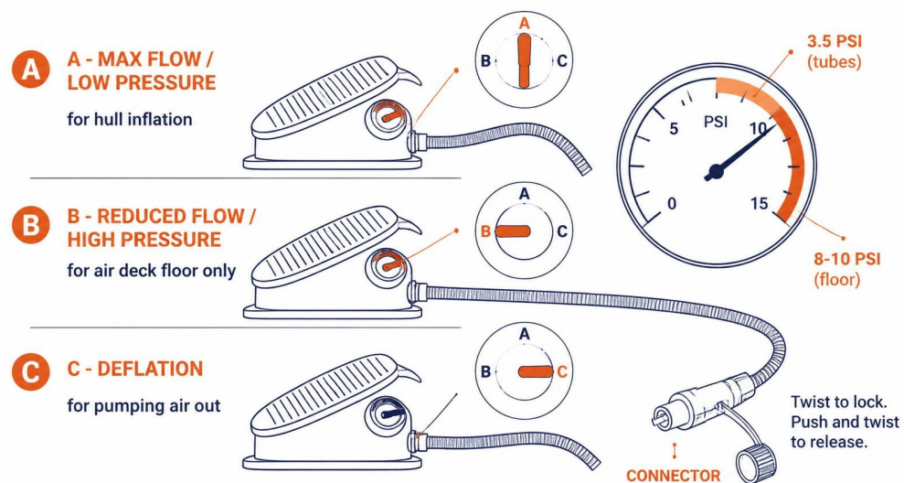
Fig. 3b · Foot pump positions A / B / C and target pressures.
