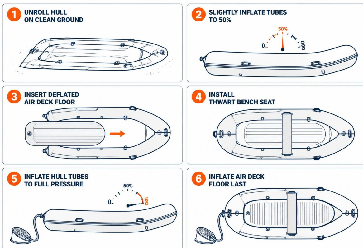
Fig. 2 · Six-step assembly sequence — hull, air deck floor, thwart, final inflation.
